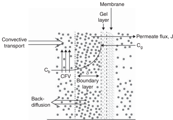
Figure 1.4 Concentration polarization.
