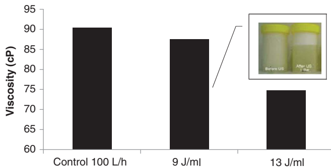
Figure 6.7 Viscosity of concentrated casein solution at 200 \text{ s}^{-1} . Sonication at 20 kHz with 11 s residence time. Insert: Appearance of foam before sonication (left) and after sonication (right) (Zisu, Kentish, Palmer and Ashokkumar, unpublished).
